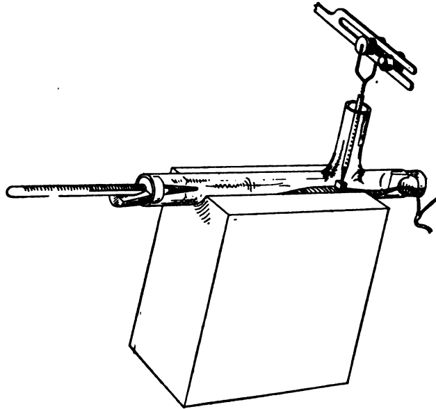
FIG. 45.—Glass chamber for controlling humidity in making auxographic record of pod of Phaeolus . Ends of horizontal part of chamber closed by cork stoppers fitted to stem of pod and thermometer. Tube to be closed around vertical arm of instrument with cotton wool.
